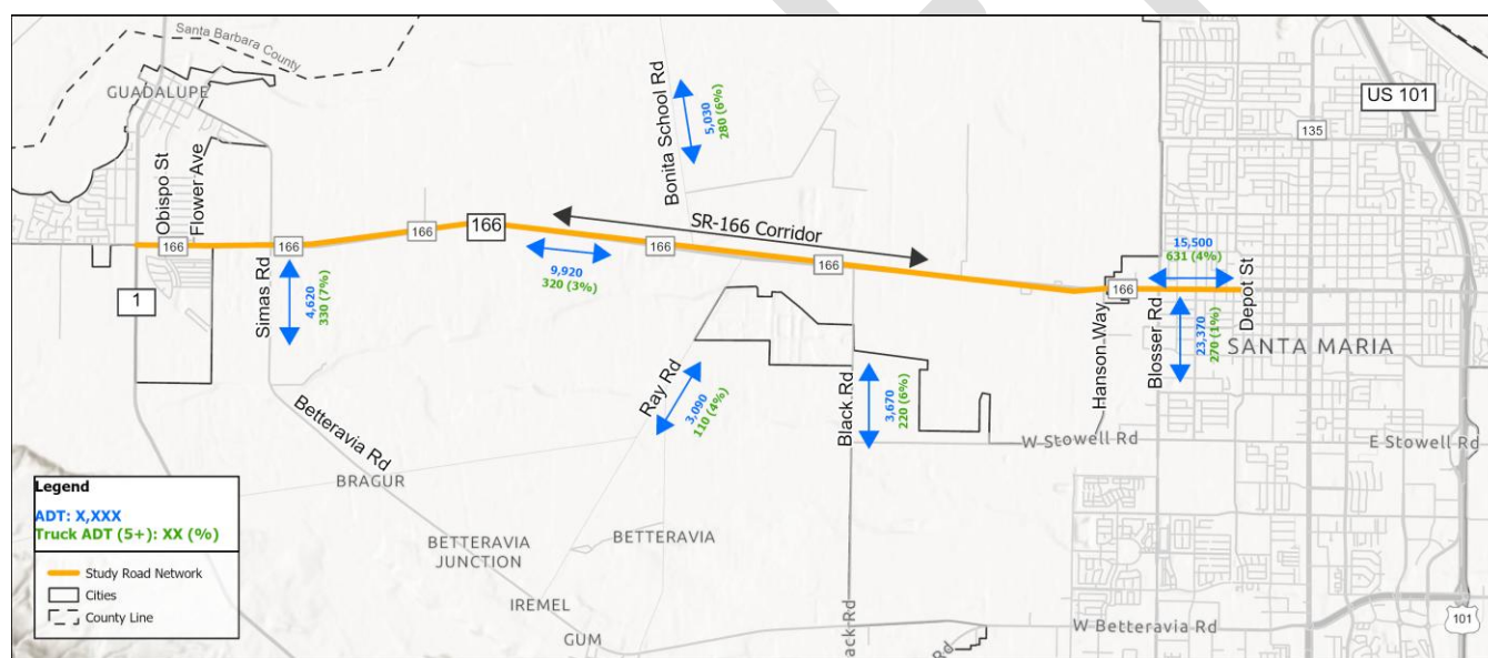
FIGURE 14: ADT AND TRUCK ADT ON STUDY ROAD NETWORK
