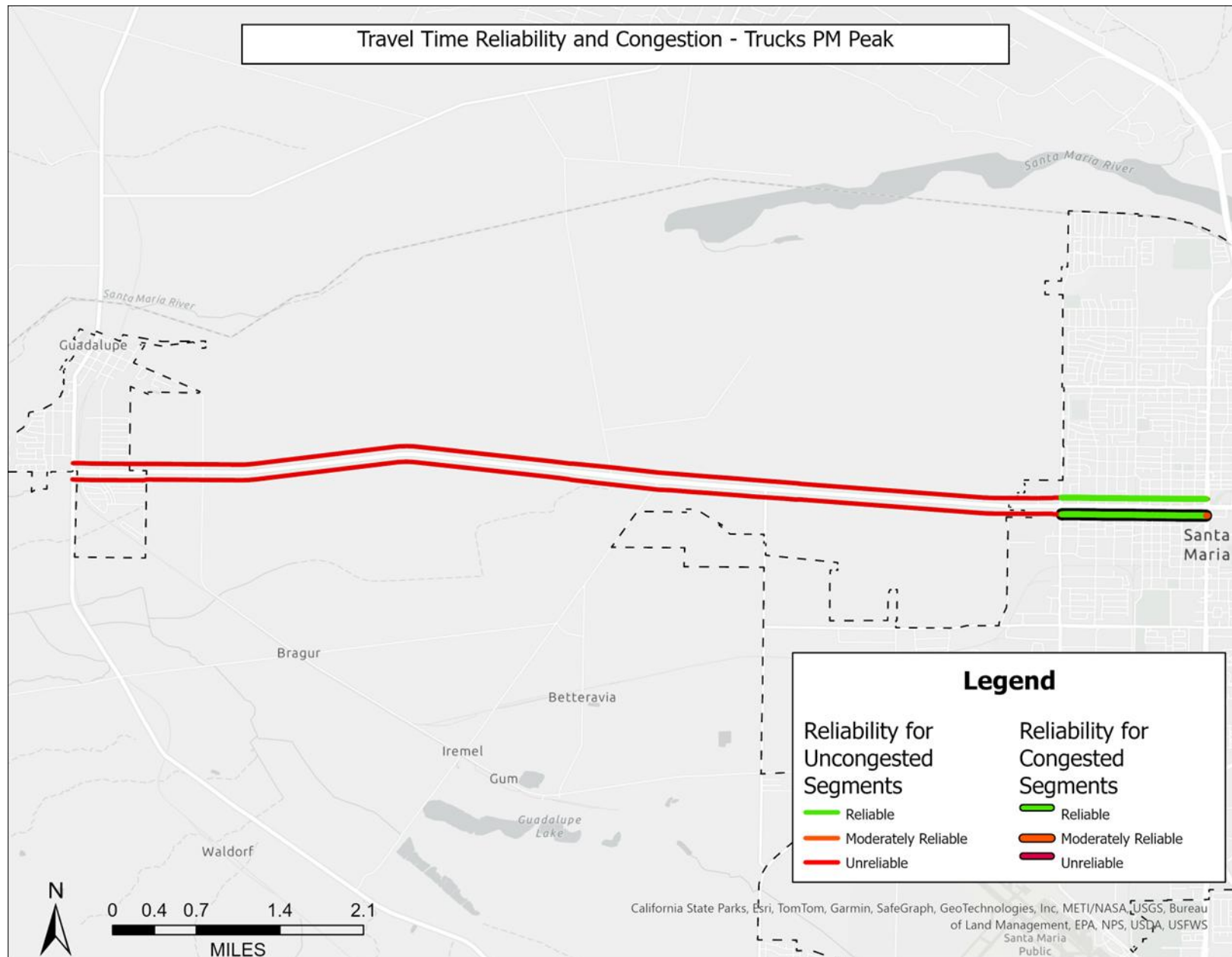
FIGURE 25. TRUCKS PM PEAK HOUR PERIOD (5:00-6:00PM) RELIABILITY AND CONGESTION
