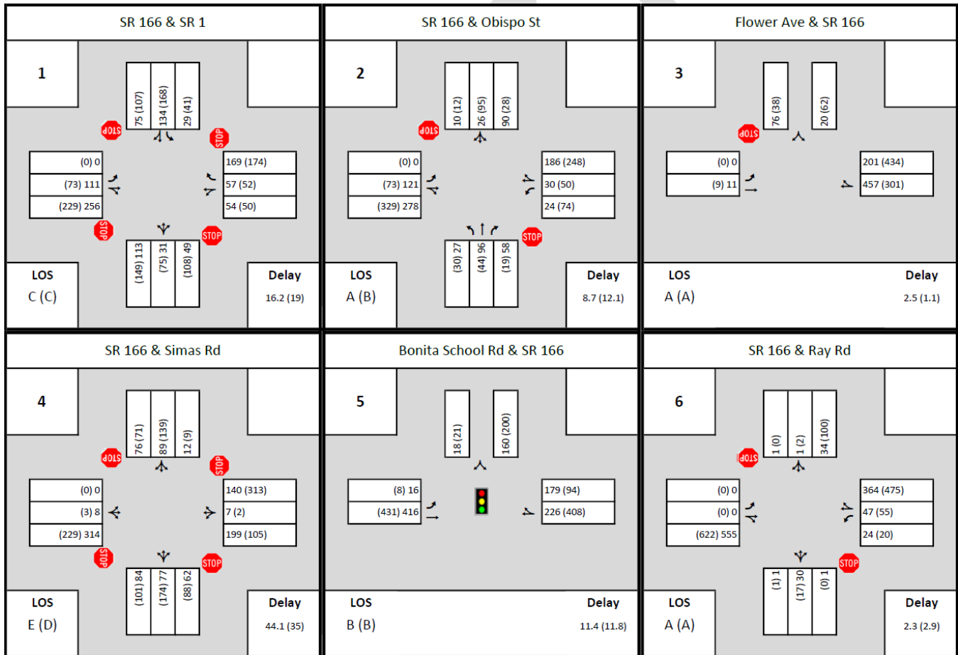
FIGURE 16: EXISTING CONDITIONS AM/PM PEAK HOUR INTERSECTION TURNING MOVEMENT COUNTS (1 OF 2)
