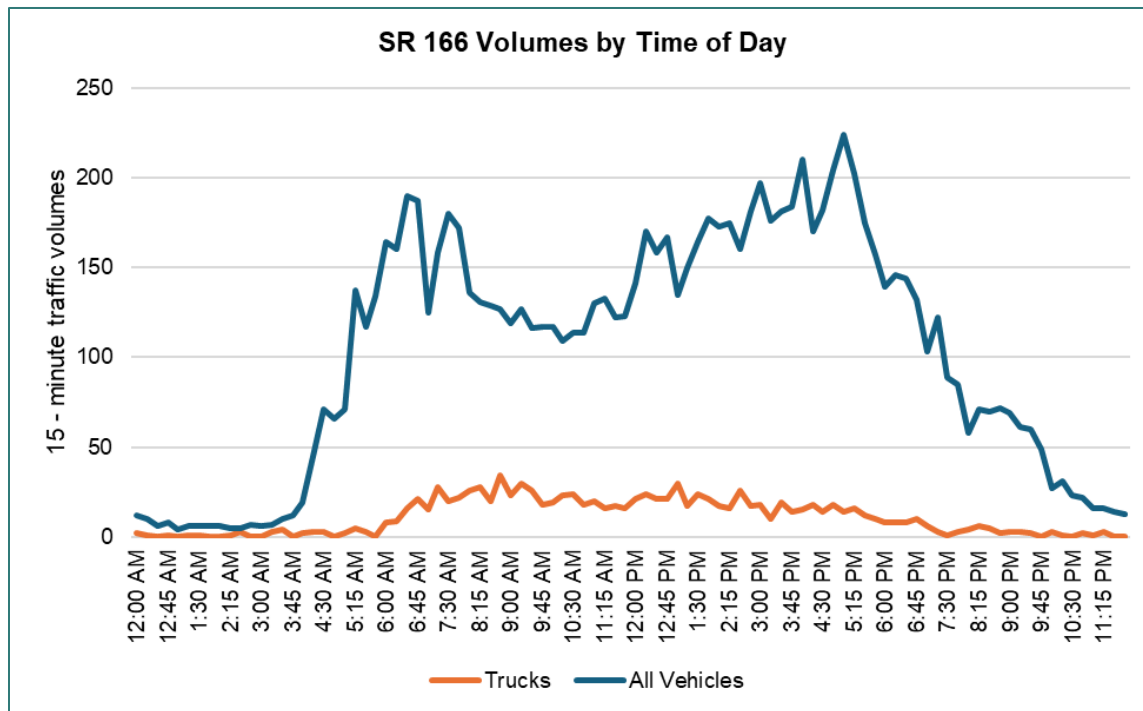
FIGURE 15: 15-MINUTE TRAFFIC VOLUMES BY TIME OF DAY
