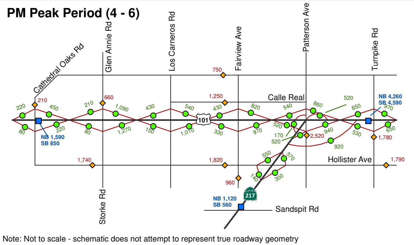
Data Collection Locations Highest Local Hourly Traffic Volumes Goleta, California
